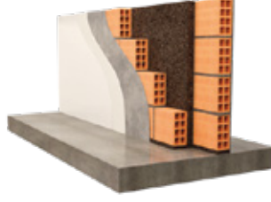
Internal partitions Double wall with insulation fully filling the cavity
